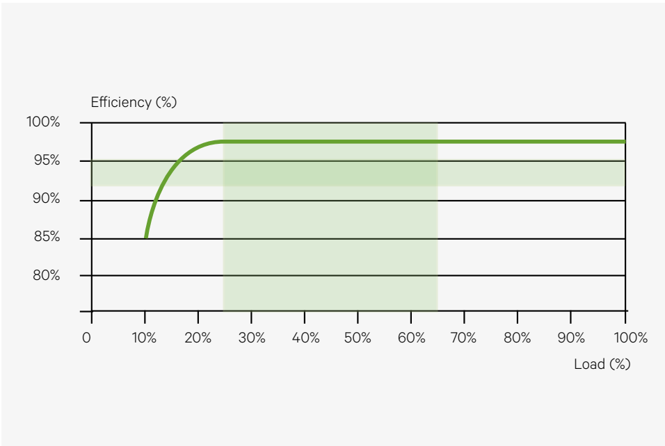
Liebert EXL S1 AC/AC efficiency with Intelligent Paralleling feature
