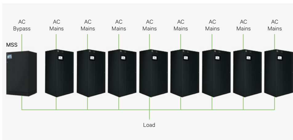
Liebert EXL S1 centralized parallel configuration, with MSS plus 8 UPS units in parallel
